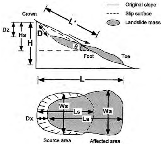
Fig. 3: Schematic geometry of a deep seated landslide and parameters. After Moriwaki and Hattaji (2002): Slope angle of source area = H_s / L_s
